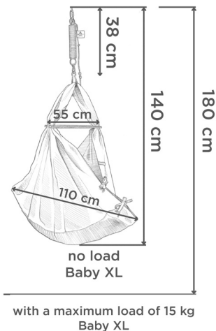
Figure 3 : DIMENSIONS OF THE CRADLE WITH SPRING UNDER DIFFERENT LOADS IN INACTIVE STATE
